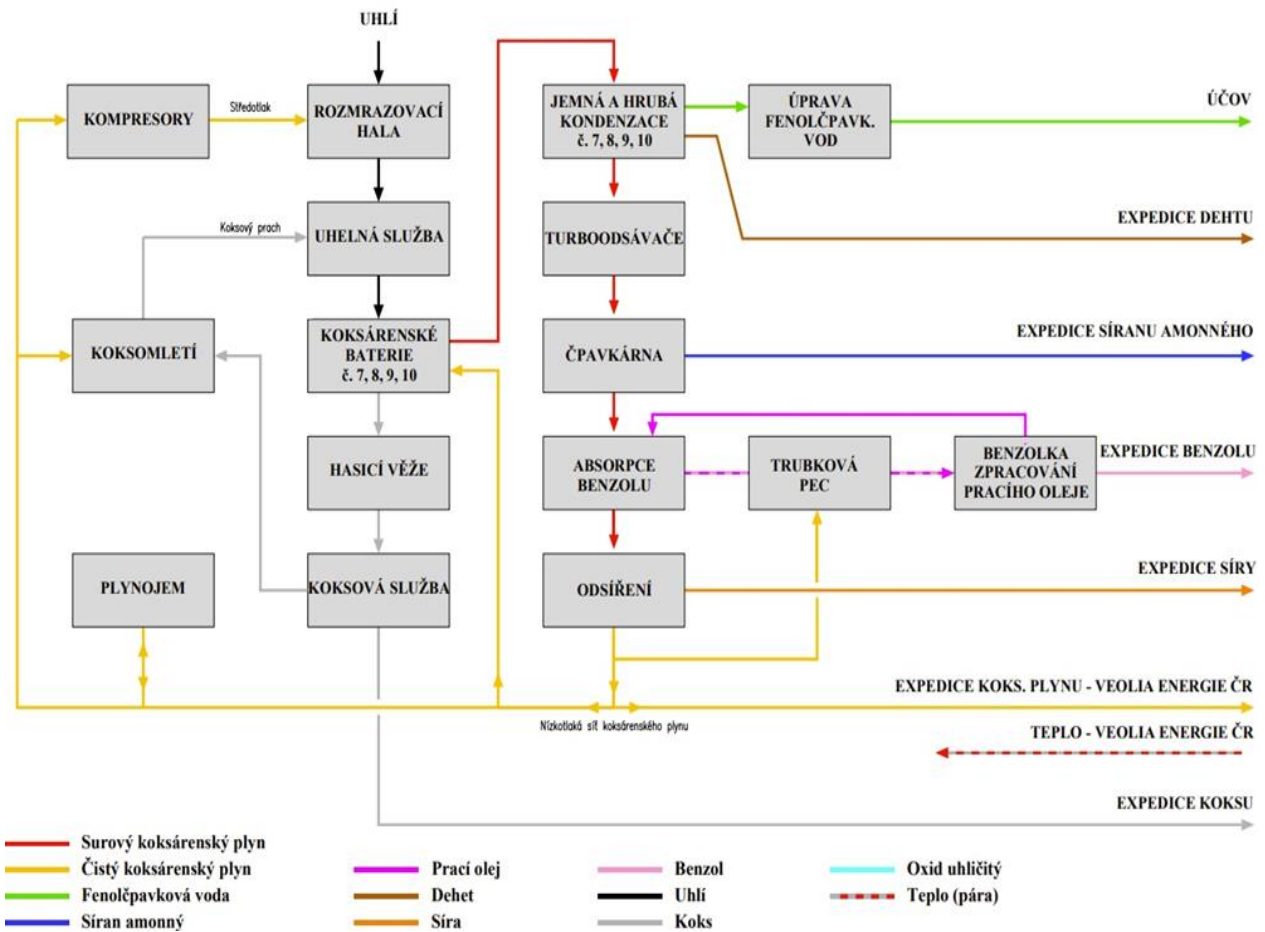
Giant. no. 1: diagram of the production process
