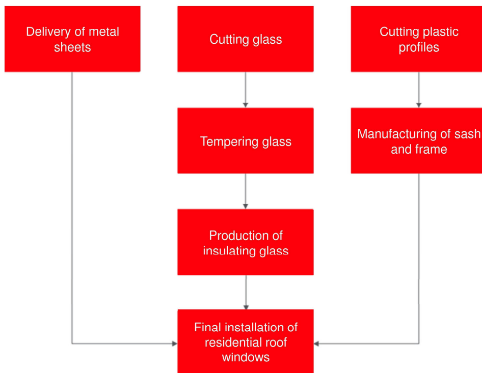
Illustration 1 Product manufacture of plastic windows
